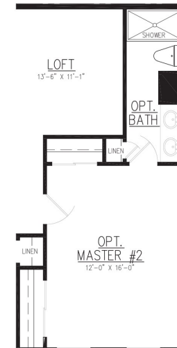
OPTIONAL MASTER BEDROOM #2 LAYOUT
