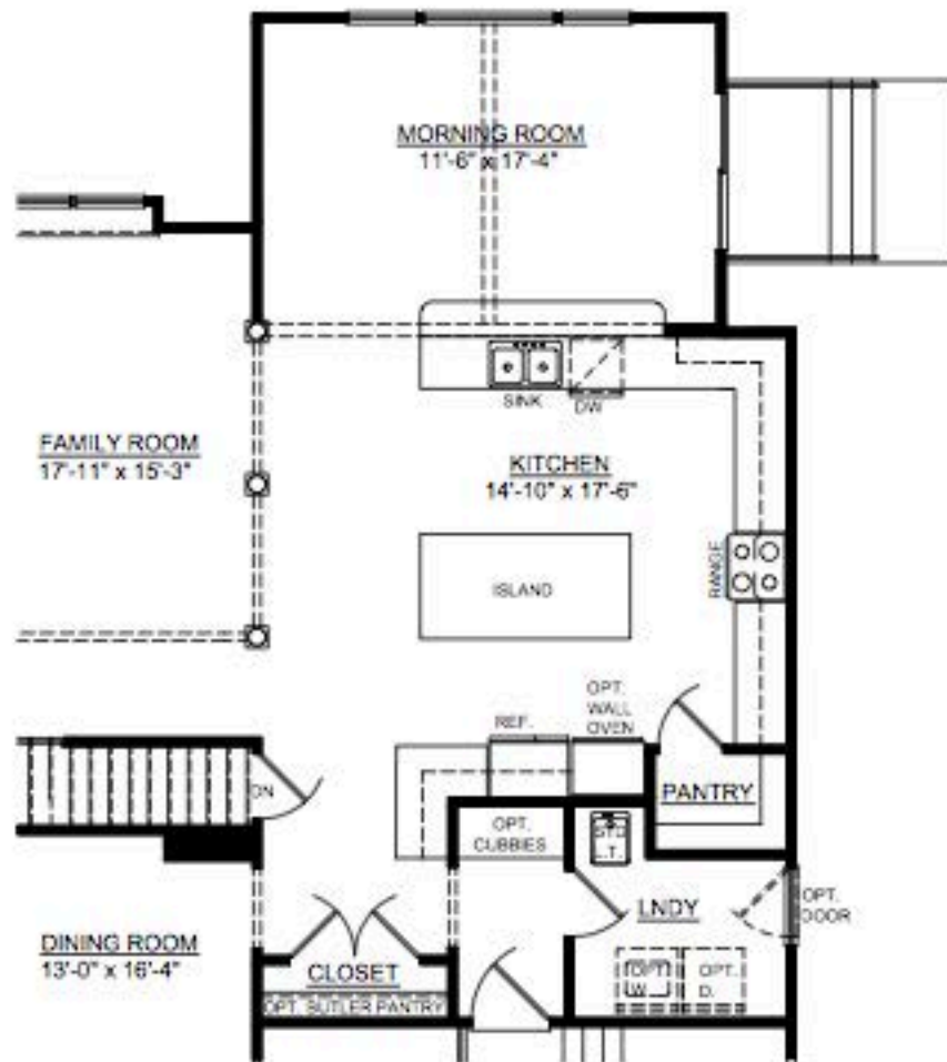
MORNING ROOM
