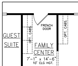
Opt. Alt. Family Center Plan
